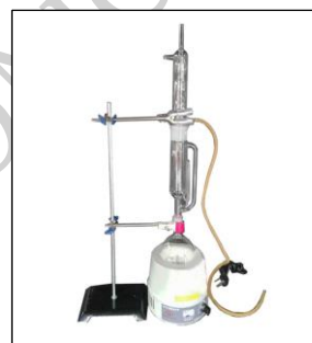
Soxhlet Apparatus
